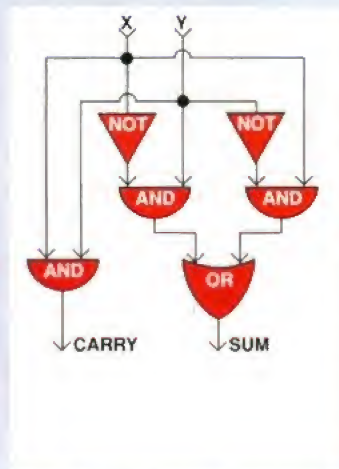
The HALF ADDER is so called because it can't handle 'carrying' a leftover digit.
